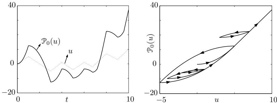
FIG. 2.3. Example of Prandtl hysteresis
