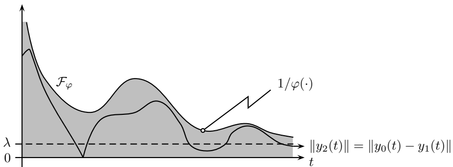
FIG. 1.3. Funnel \mathcal{F}_\varphi with \varphi \in \Phi and \inf_{t>0} \varphi(t)^{-1} = \lambda
