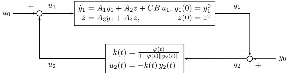
FIG. 1.2. The “funnel controlled” closed-loop system.
