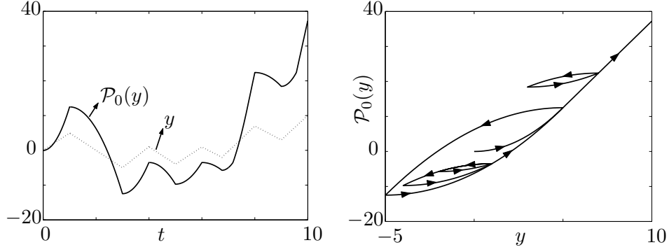
Figure 9: Example of Prandtl hysteresis
