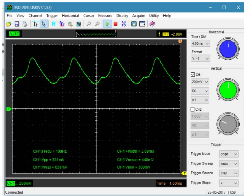
LED Lamp – sample 2 - CELED, 7W, 230V, R_a=80 , 500lm, 25000h, warm light 2700-3000K
