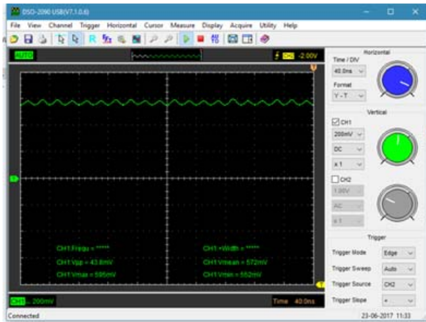
LED Lamp – Sample 7 - Neolux, 9.5W, 230V, Ra=80, 806lm, 15000h, warm light 2700K
