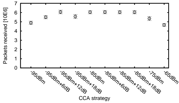
Figure 10: Number of received CAMs in Millions.
