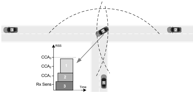
Figure 2: Accumulated signals result in interference at transmitter T . Clear channel only indicated if CCA_3 is applied.
