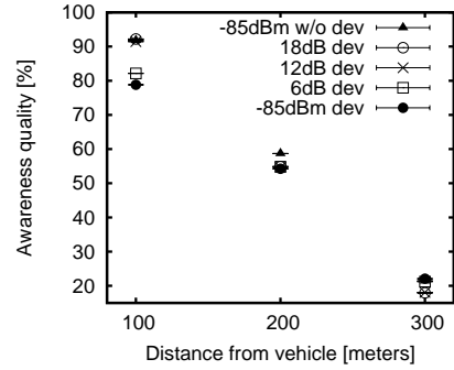
Figure 11: Awareness quality for 100, 200, and 300 meters under inaccuracies of the CCA threshold.
