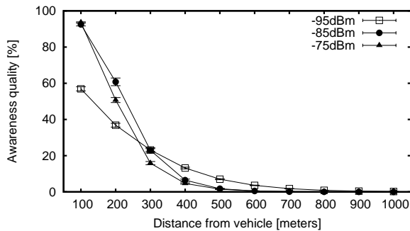
Figure 7: Awareness quality for static CCA thresholds in high channel load.
