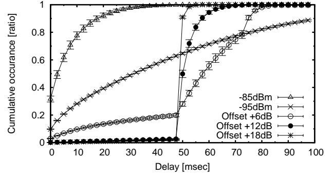
Figure 9: Average medium access delay a) and cumulative distribution b) for -95 dBm base CCA threshold.
