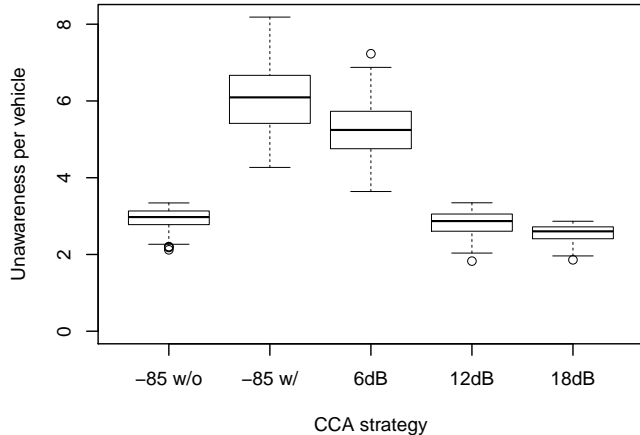
Figure 12: Awareness quality under inaccuracies of the CCA threshold.
