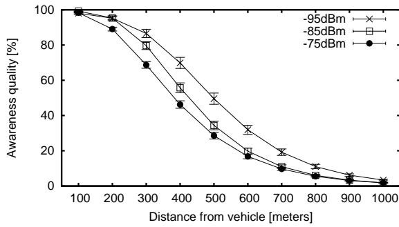
Figure 5: Awareness quality for static CCA thresholds in a) low channel load and b) medium channel load.
