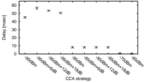
Figure 9: Average medium access delay a) and cumulative distribution b) for -95 dBm base CCA threshold.
