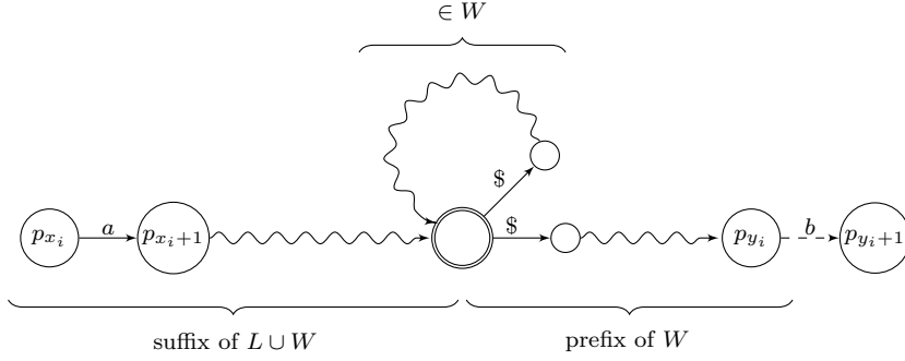
Fig. 1 A run labeled with v_i from p_{x_i} to p_{y_i} in \mathcal{C} .
