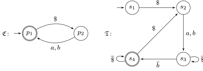
Fig. 2 NFAs \mathfrak{C} and \mathfrak{T} accepting LW^* and (W\bar{R})^* , respectively, from Example 5.7.
