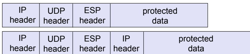
NAT-T packet structure – Transport and Tunnel Mode
