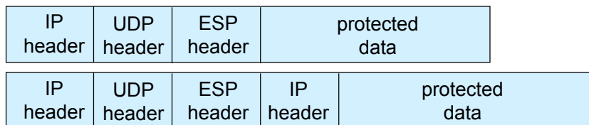
NAT-T packet structure – Transport and Tunnel Mode
