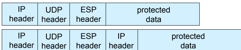
NAT-T packet structure – Transport and Tunnel Mode
