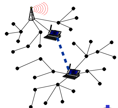
Wormhole Attack
