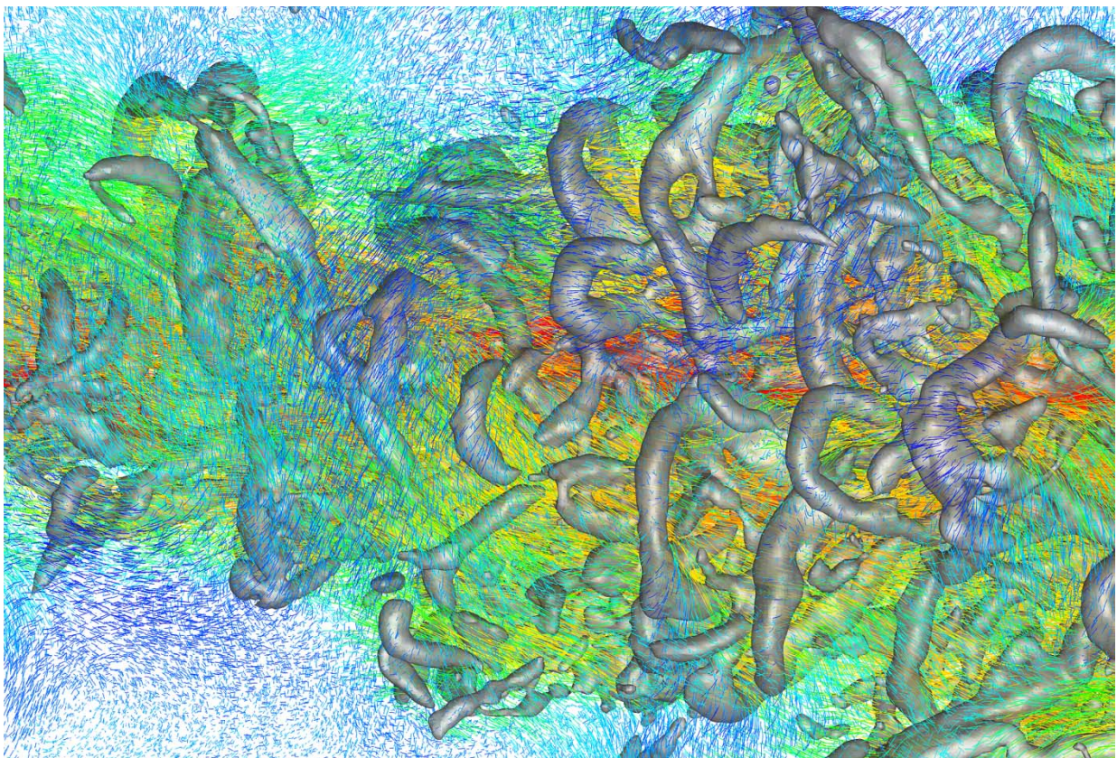
Figure: Thermal plume (tilted by 90°) with Lagrangian tracks of ~300,000 particles in a 0.6 m 3 volume, color coded with vertical velocity. Isosurfaces of Q-criterion show vortical structures.
