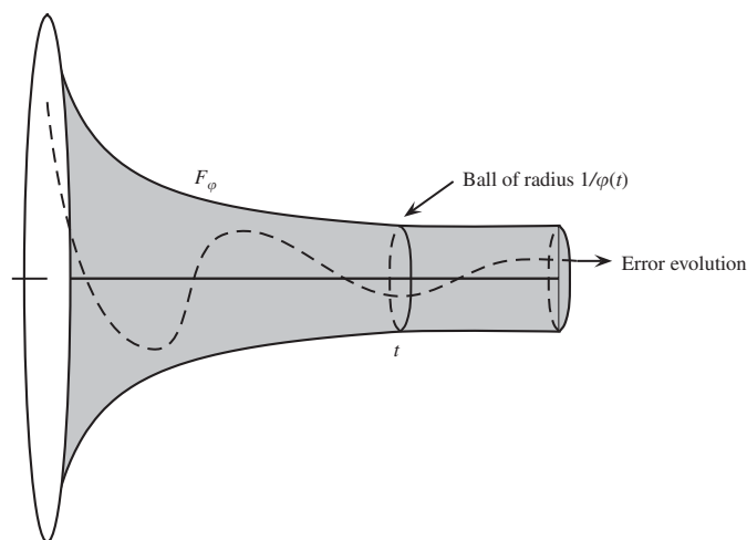
Fig. 1. Prescribed performance funnel \mathcal{F}_\varphi .
