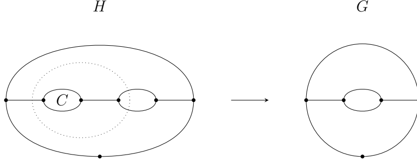
Figure 2: Contraction in the proof of Lemma 3 (i)
