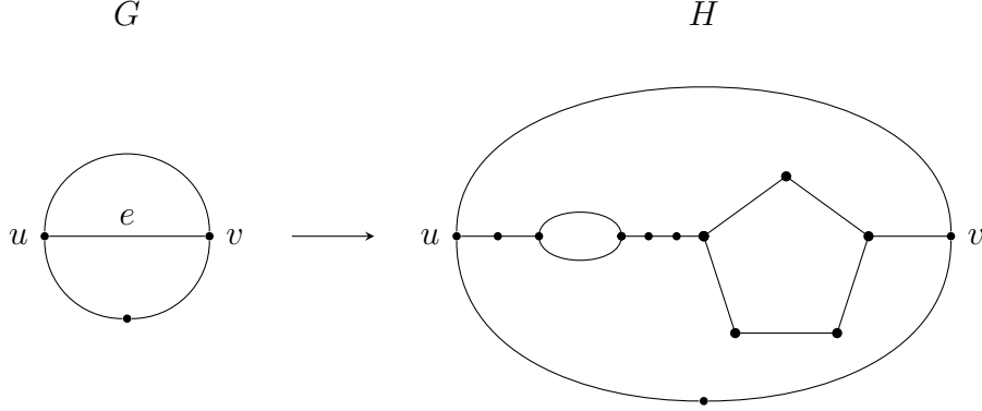
Figure 1: Replacing the edge e = uv \in E(G) with a 2-cycle-chain
