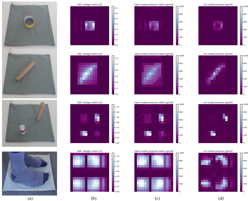
Fig. 9. Examples of real pressure patterns captured with the 16x16 sensor array. (a) These objects have been pushed down on the sensor with increasing weights in order to generate the input patterns, (b) The ADC voltage matrix measured with a mid range weight, (c) Result using the naive approximation ignoring parallel pathways in the matrix, (d) Results of the CNN approach showing improved and better fitting shapes of activation.
