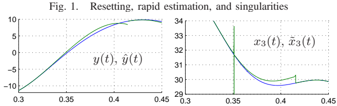
Fig. 1. Resetting, rapid estimation, and singularities
