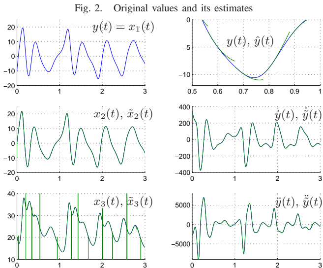
Fig. 2. Original values and its estimates
