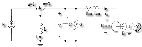
Fig. 1. The combination ‘‘dc Motor-Buck-Boost-power-converter’’ model
