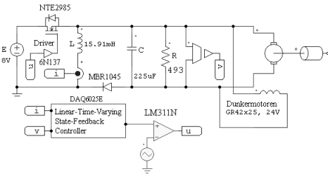
Fig. 2. Experimental set-up for the “Buck-Boost” converter-dc Motor with linear-time-varying state feedback controller
