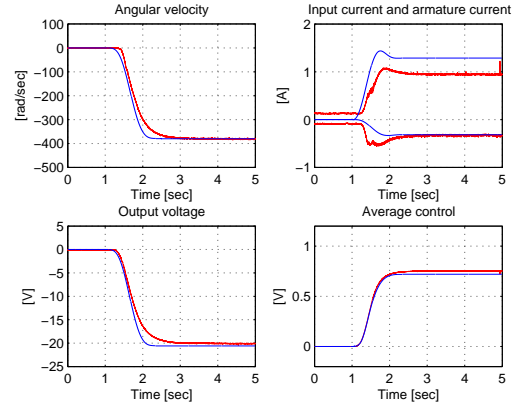
Fig. 3. Angular velocity, input current, output voltage and average control input response for a desired angular velocity trajectory tracking task
